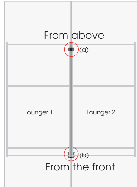
Fixation with 2 connector clips (VB1)
