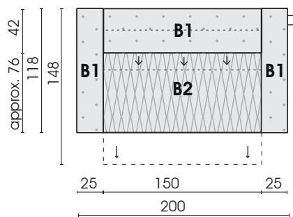
Sofa 2,5-seat, 2 AR functional back, motorised seat adjustment 24MF
