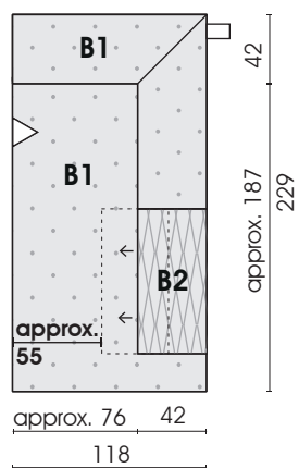
Corner sofa 3-seat, right functional back, fixed corner 345F
