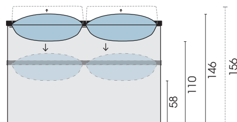
Element 2,5-seat without armrest functional back R22, incl. motorised traverse
