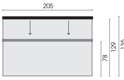
Element 2,5-seat incl. motorised traverse 49M
