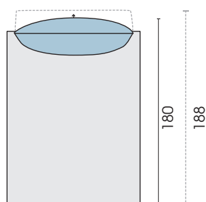
Lounger, functional back R05 incl. fixed traverse
