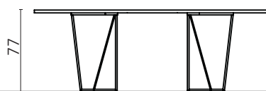
Front view, type T220HG/T220S
