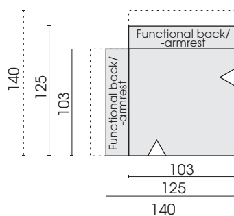
Corner element deep with functional back/-armrest 70T
