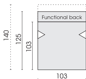
Element deep with functional back 13T
