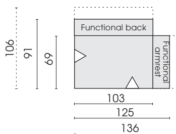
Element with functional armrest, right and functional back 110
